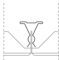
BANDEJA CAPRI (CLIP-IN)
